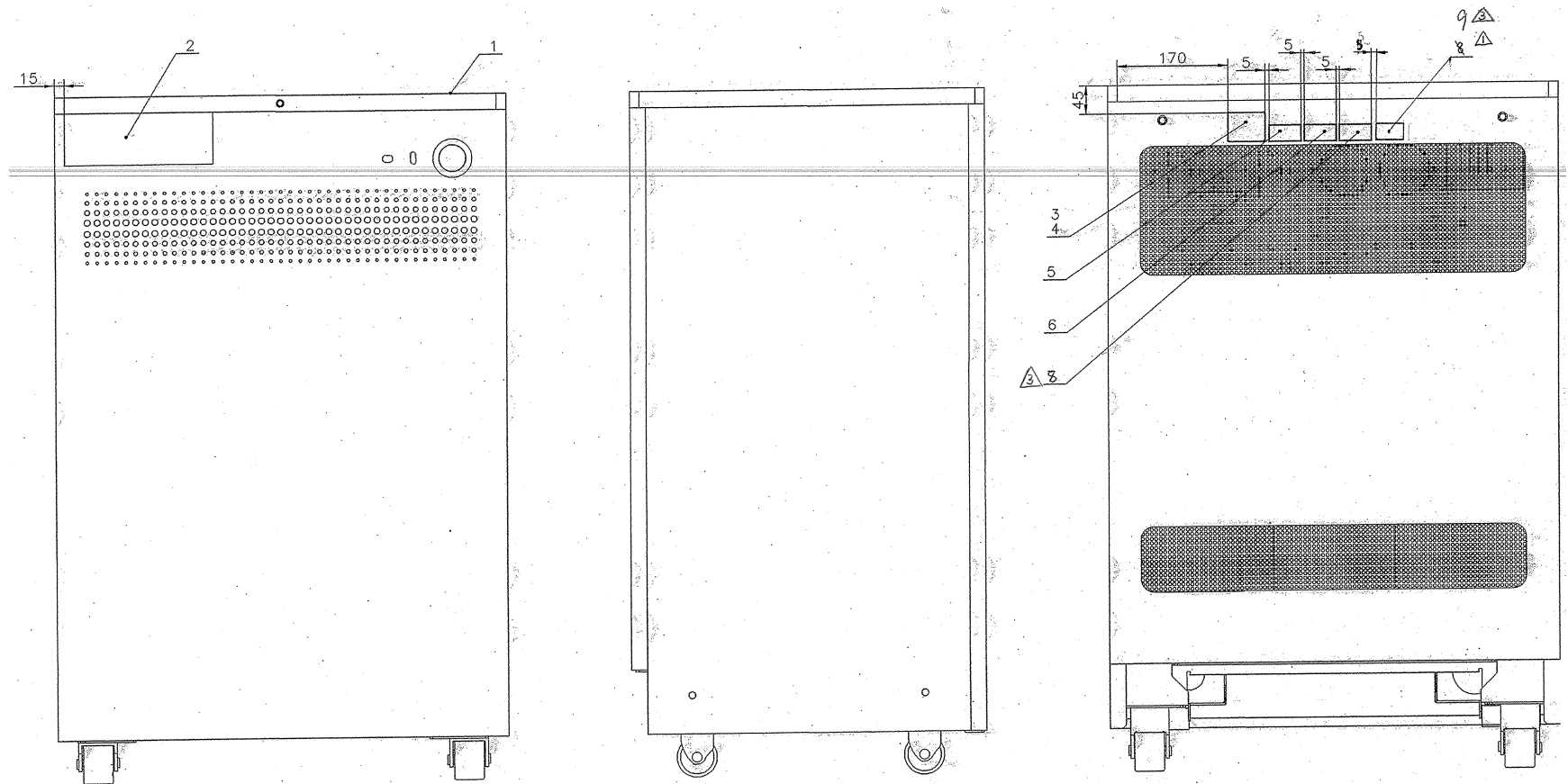
Figure 3-1 NGPDU-4 Assembly (2326492-4 Sheet 2, Rev 4)
