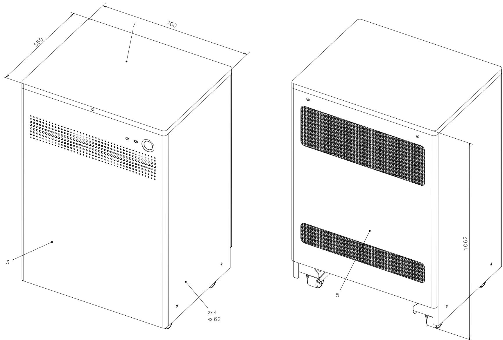
Figure 3-2 NGPDU Assembly 4 (5125934, Sheet 1, Rev 4)
